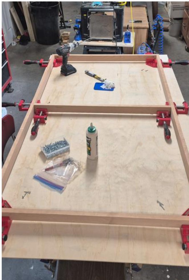
Part of a frame being assembled.
